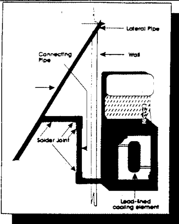
Water Cooler
