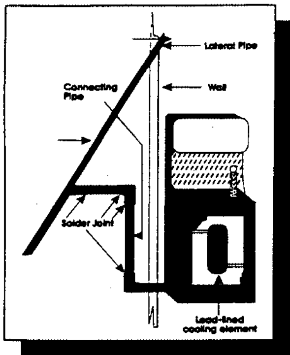
Water Cooler
