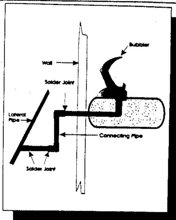
Bubbler
